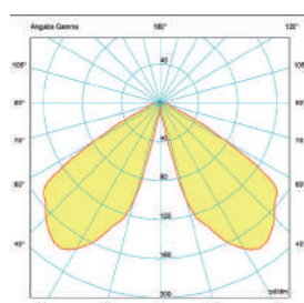
SBE500 LED
