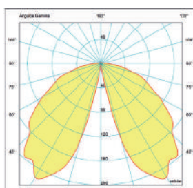
SBT400 LED
