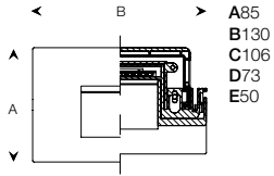
Scatola 503 Recessed box
