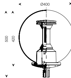
SFERA COMPLETA TRASPARENTE IP65 COMPLETE TRANSPARENT GLOBE IP65
