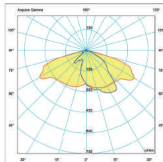
96W 12900lm
