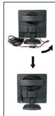
Wiring system
